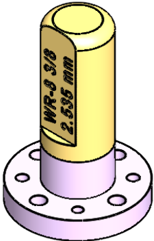
WR-8 WAVEGUIDE OFFSET
